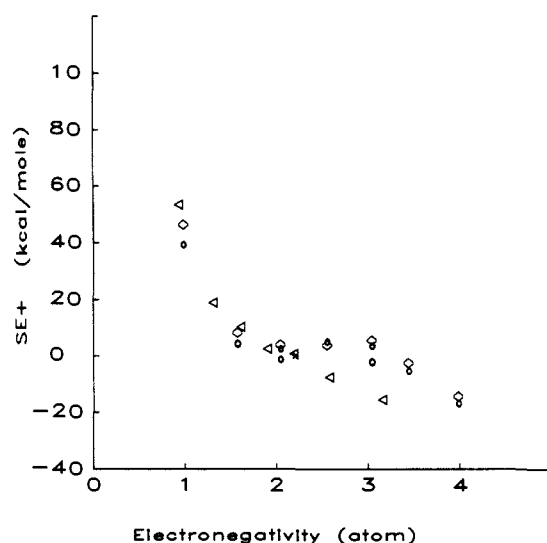
Figure 1. (a) Stabilization energy (kcal/mol) of PER \beta -substituted ethyl cations versus Pauling electronegativity of the non-hydrogen atom of the substituent: X = hydrogen substituent; \diamond = second-row substituents; \Delta = third-row substituents; O = Apeloig et al. 3 second-row data, 4-31G basis set. (b) Stabilization energy (kcal/mol) of PLA \beta -substituted ethyl cations versus Pauling electronegativity of the non-hydrogen atom of the substituent.
